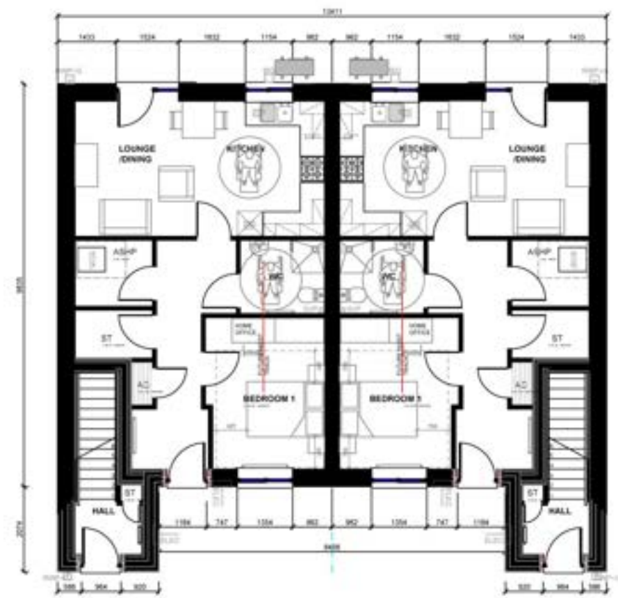
GROUND FLOOR PLAN FFLAT 2P1B
